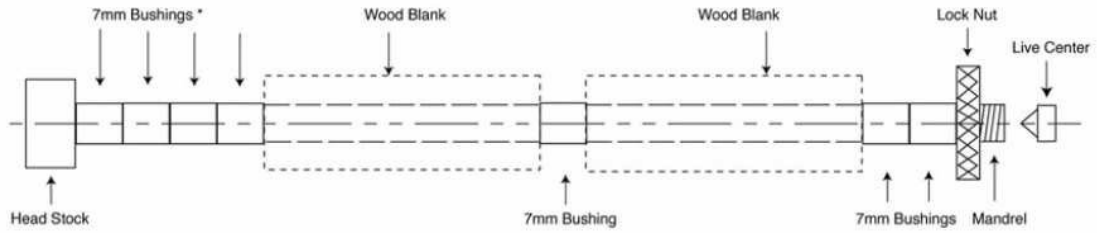
Diagram B - Turning the Blanks
