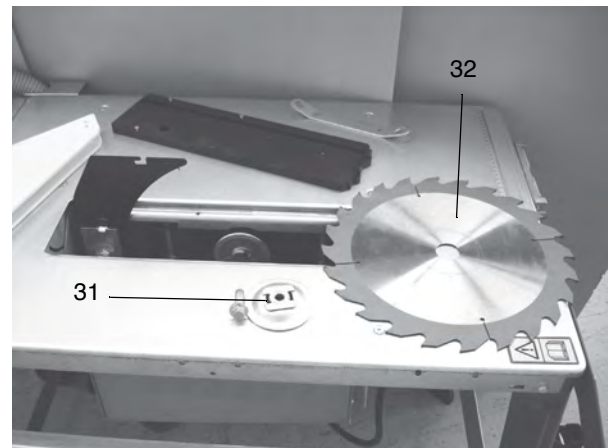
Fig. 40: Mount saw blade flange
